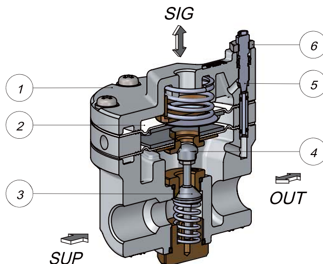
< Sectional View of AVB-2000 >
