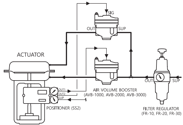
DOUBLE ACTING
