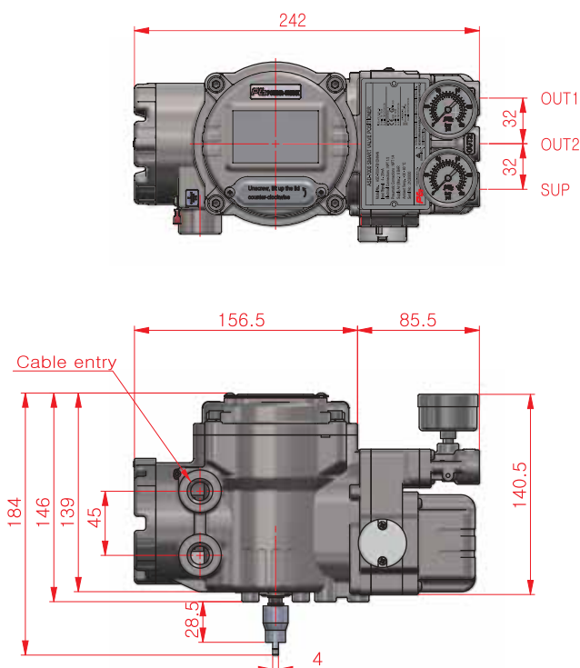
ASD-7010 Rotary type
