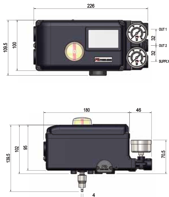
ASD-5010 Rotary type
