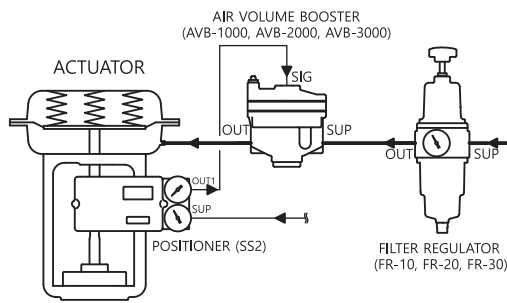
SINGLE ACTING
