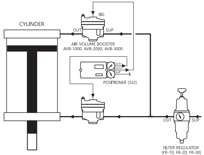
CYLINDER ACTUATOR
