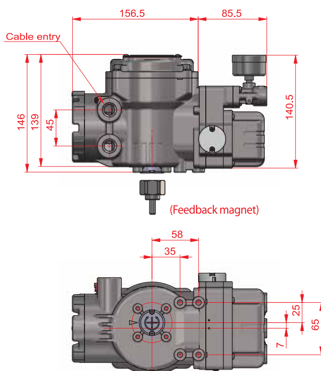
ASD-7011 Rotary type
