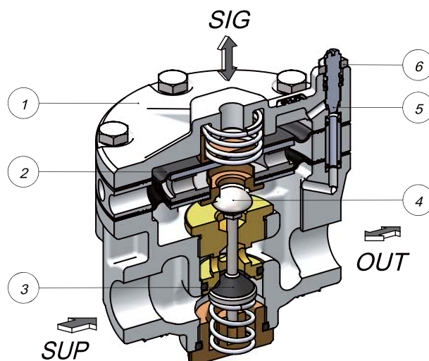
< Sectional View of AVB-3000 >
