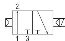
ESV-32 < Normally - open >
