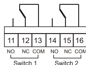
Micro switches 1, 2
